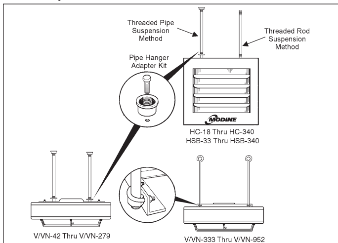
Figure 5.1 Unit Suspension
